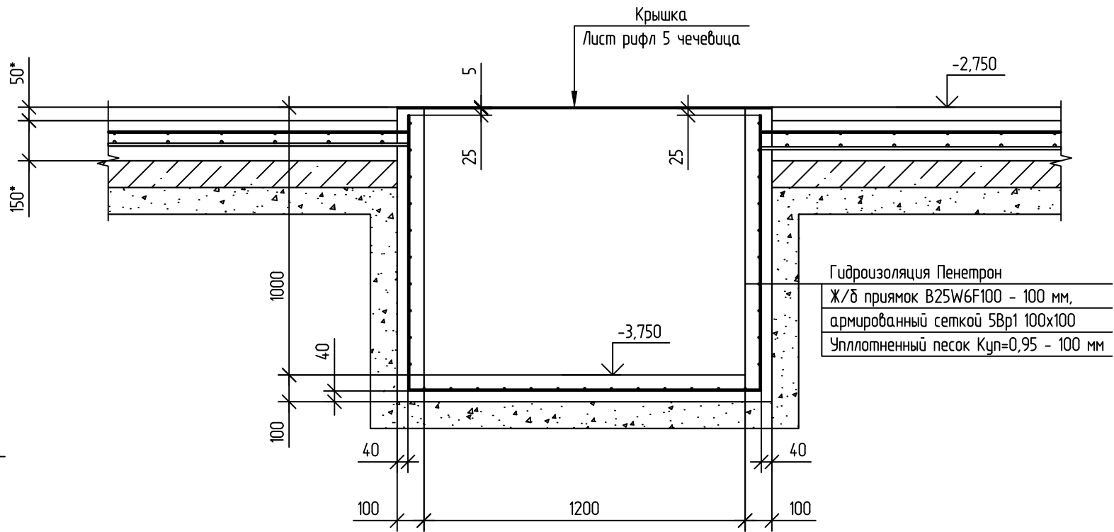
Схема прямка ПР-1 (1200x1200x1000)
